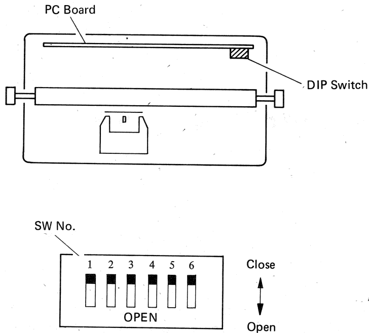
Figure 10. DWP-210 DIP Switch Settings
