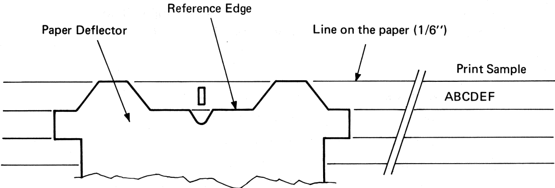
Figure 9. Print Position
