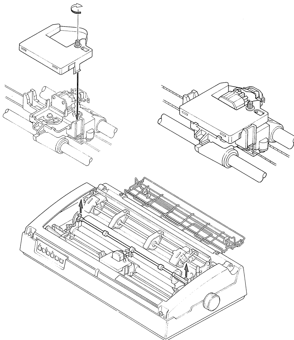
Figure 9. Installed Ribbon Cassette
