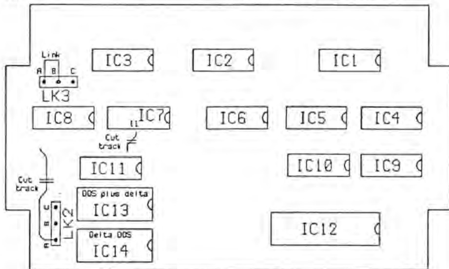
Delta DOS cartridge layout
