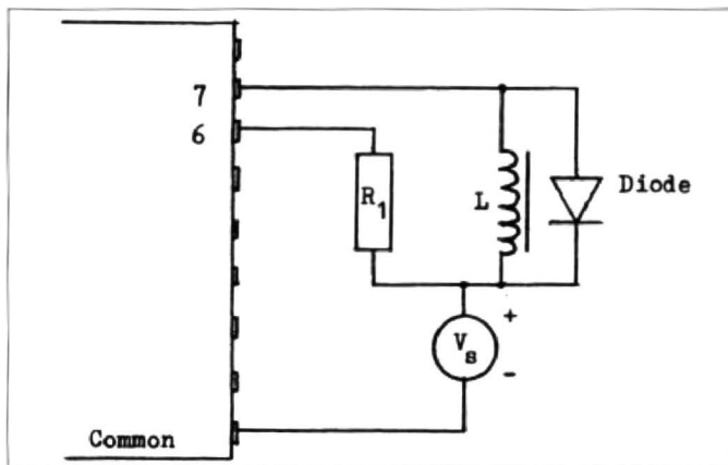
Figure two: connections for an inductive load
