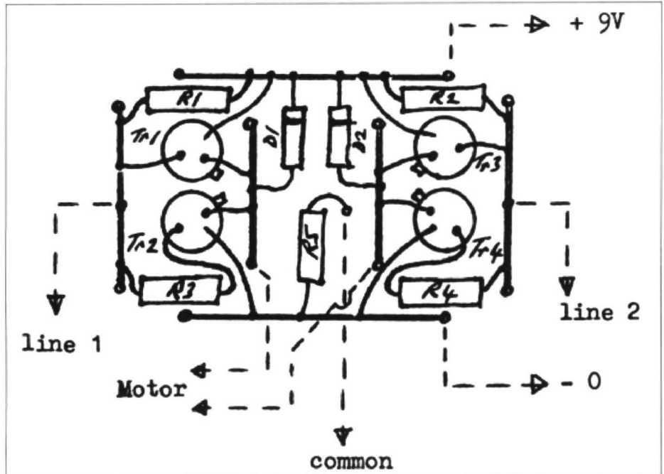
Figure nine: a component layout for the circuit board.
