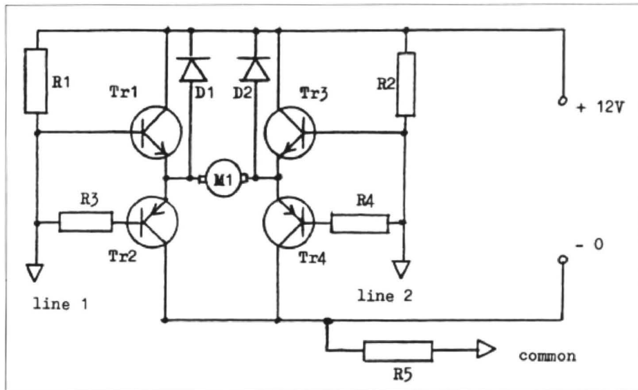
Figure six: a basic bridge circuit.
