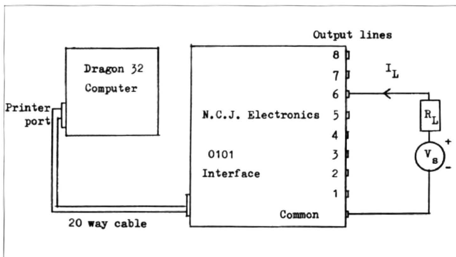
Figure one: the generalised interface connections.
