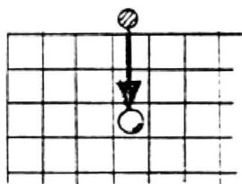
Figure 1: simple absorption
