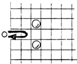
Figure 3: reflection
