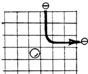
Figure 2: simple deflection
