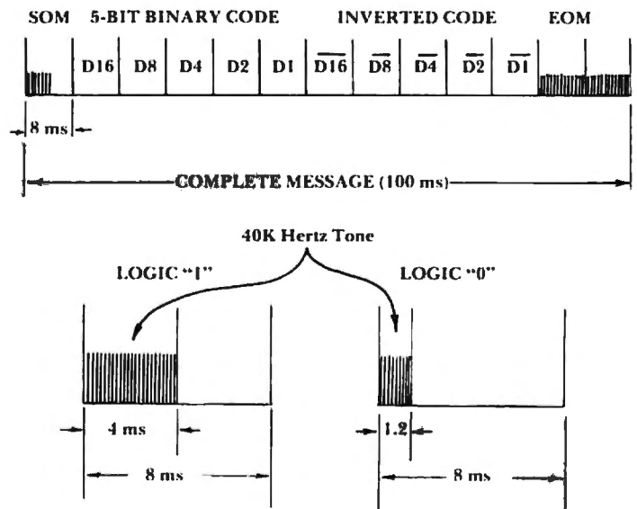
Figure 1: Description of coded message sent from cordless controller to the command console.
