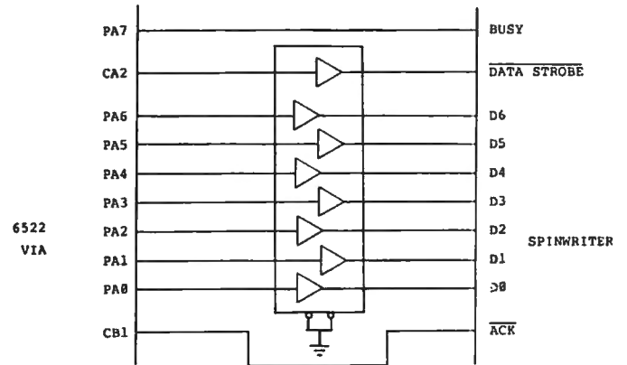
Figure 3. Connection from VIA to Spinwriter.
