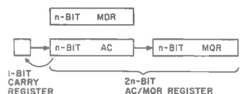
Figure 3. Multiplier register structure.
