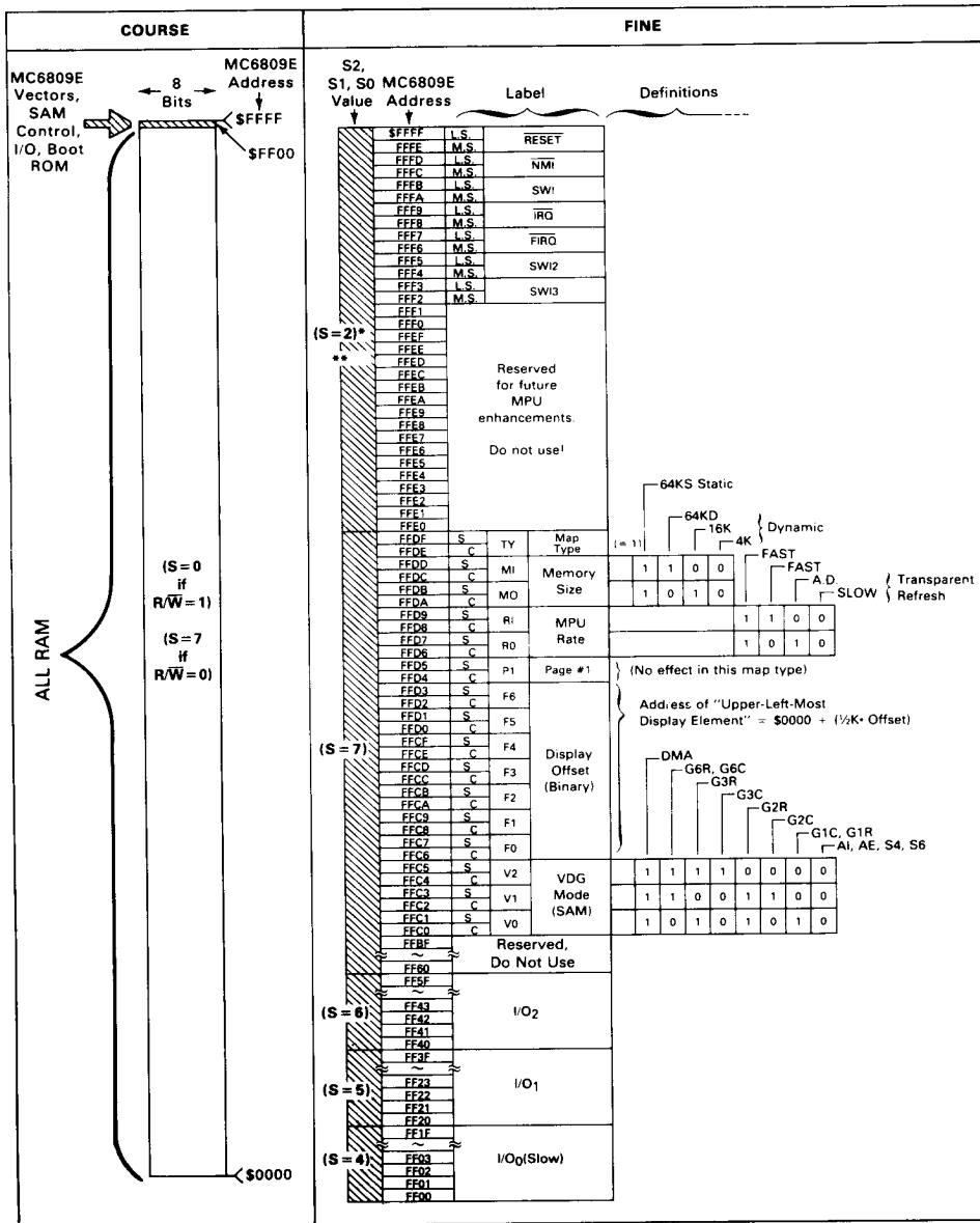
FIGURE 16 — LS785 MEMORY MAP (TYPE #1 64K RAM)
