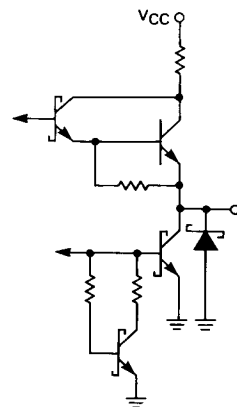
FIGURE 23 — TYPICAL OUTPUT
