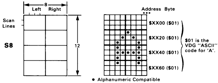
FIGURE C1 — DISPLAY MODES S8, S12, S24 Bit/Visible Dot Correlation
