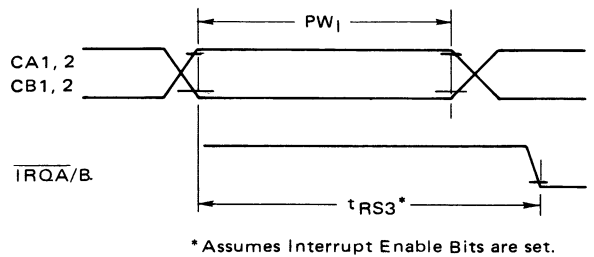
FIGURE 13 — INTERRUPT PULSE WIDTH AND \overline{IRQ}/B RESPONSE
