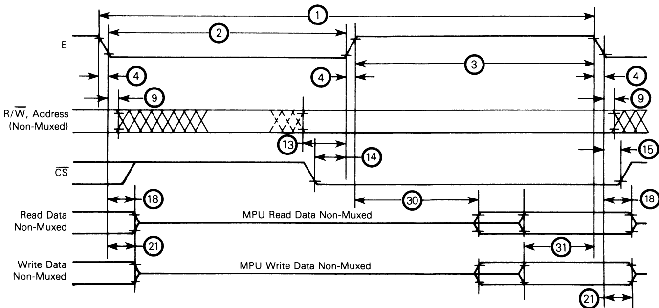
FIGURE 1 – BUS TIMING
