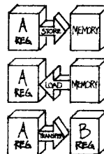
6809 DIALECT
