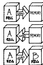
Z80 DIALECT
