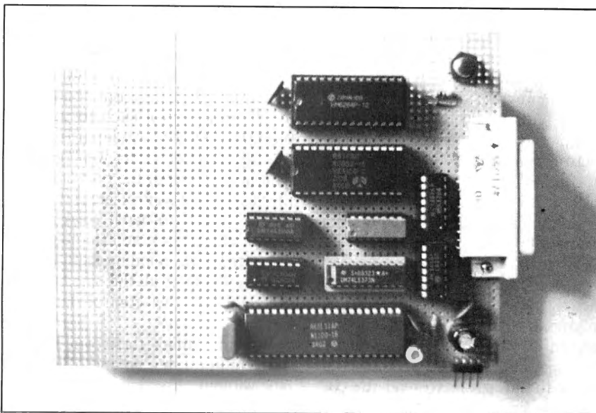
Photo. The Forth Microcontroller.
