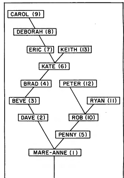
Figure 2. A graphic representation of a binary tree sort. The numbers refer to the order in which the user entered the names.
