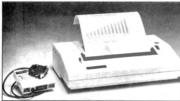
The Alphacom Traveler thermal printer uses NiCad batteries.
