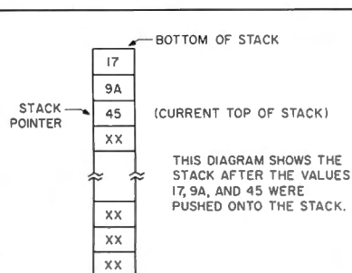
Figure 6. Illustration of a stack in memory.
